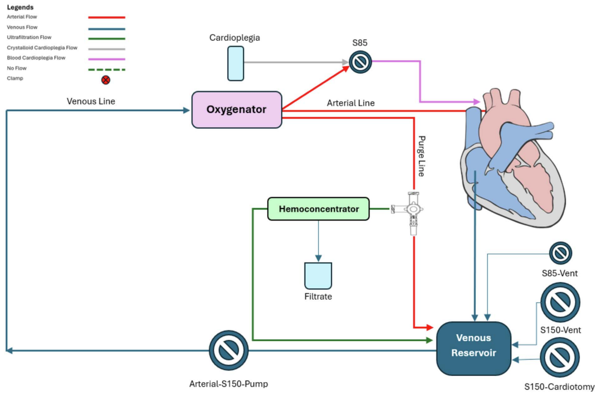
Figure 2. Conventional ultrafiltration (CUF): Hemofilter inflow connected to oxygenator purge line; outflow to venous reservoir.
